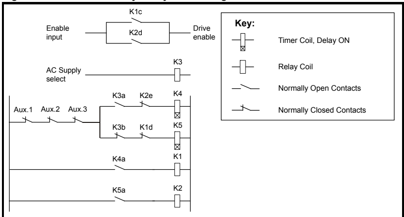
Figure 4-6 Control circuitry for system configuration 2
