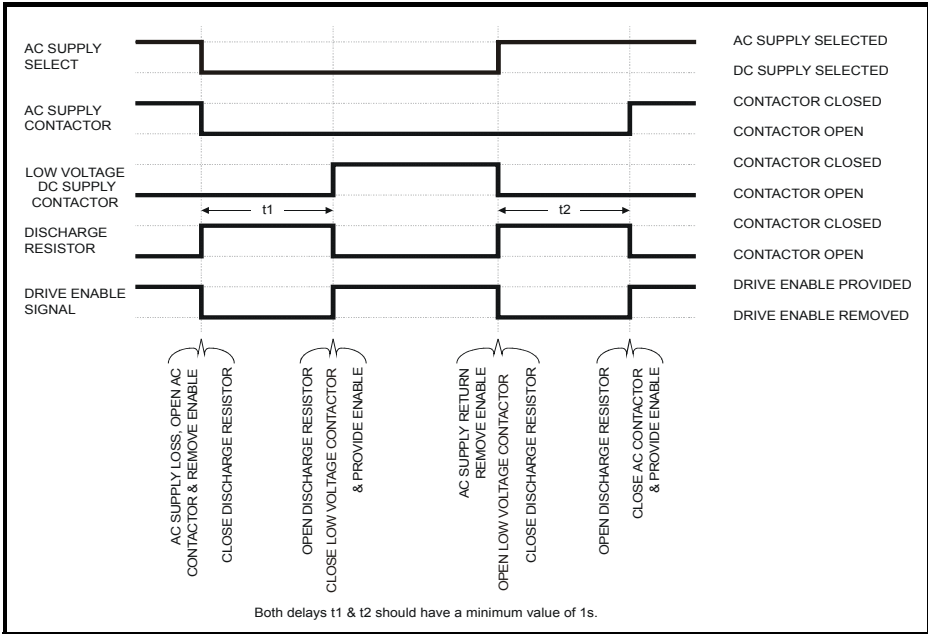
Figure 4-10 Control logic and sequencing
