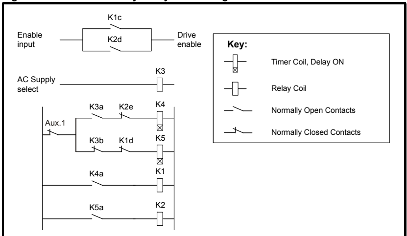
Figure 4-2 Control circuitry for system configuration 1
