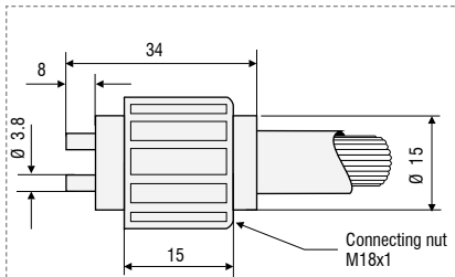
Adapter, FA System FASOP
