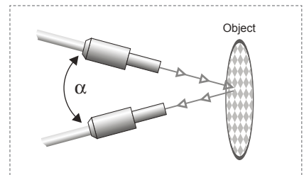
D Transmitted light operation (V arrangement) for reflective and shiny surfaces
