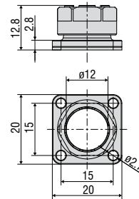
Mounting flange (optional)
