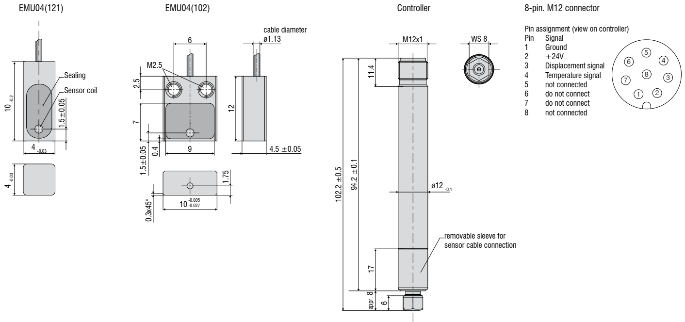
Connector (max. 20 mating cycles possible)
