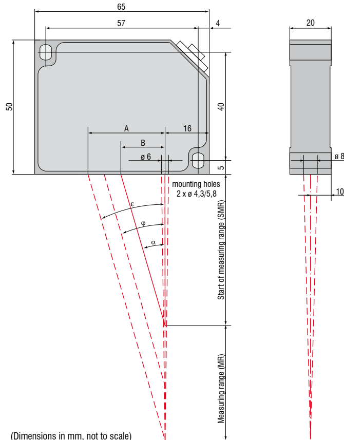
(Dimensions in mm, not to scale)
