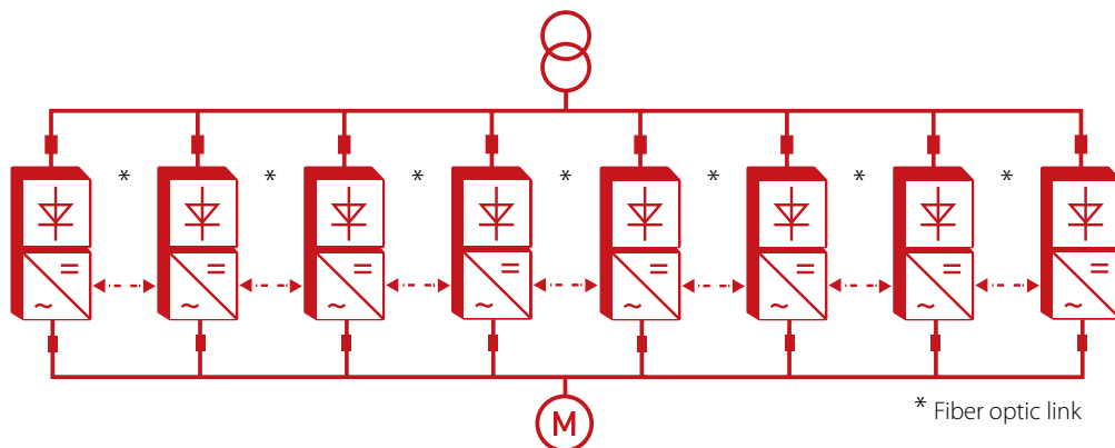
Example of the VACON® DriveSync configuration.
