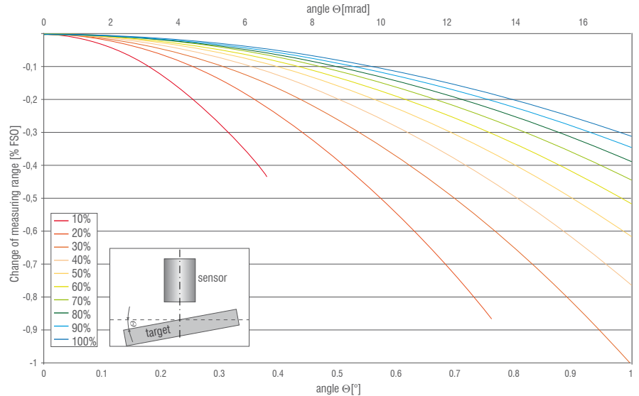
Angle dependence with different offset distances (sensor CS02)
