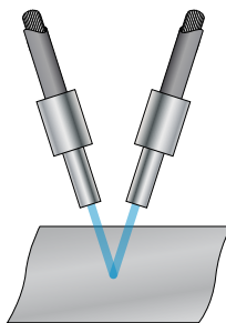
V arrangement in reflex mode
