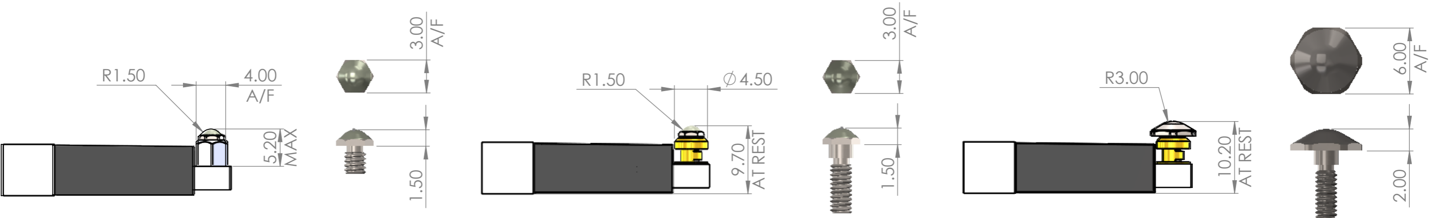
TYPE 'Y' FIXED TIP ASSY VERSION
