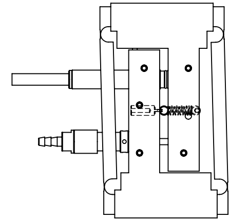
AU/1/P(H) OR DU/2/P STANDARD
