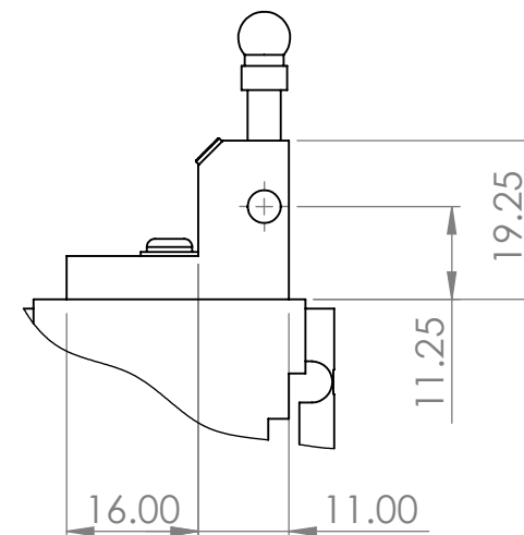
TOOL HOLDER - ASSEMBLED
