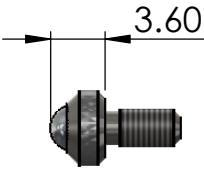
802605 - BALL TIP T/C METRIC (M2.5) *OLD DESIGN*
