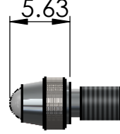
806794 - BALL TIP NYLON UNF (4-48) *NEW DESIGN*
