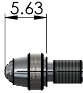
806793 - BALL TIP T/C UNF (4-48) *NEW DESIGN*
