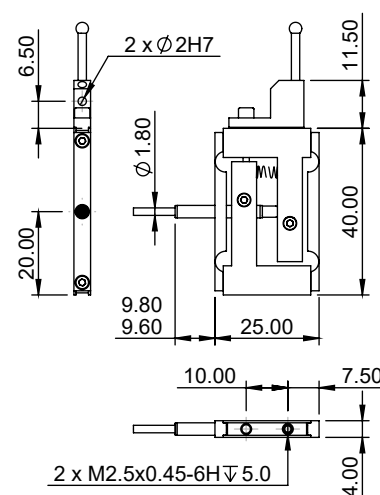
Miniature Flexure Gauge (DU/0.5/S)
