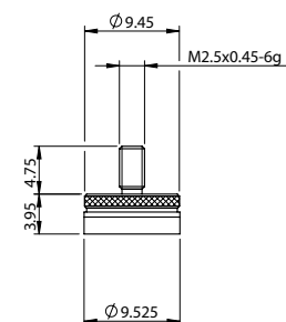
Ø9.52 mm Flat
