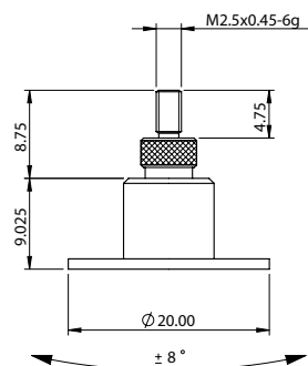
Floating Tip
