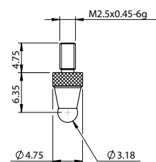
Ø3.18 mm Ball
