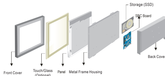
Mechanical design
