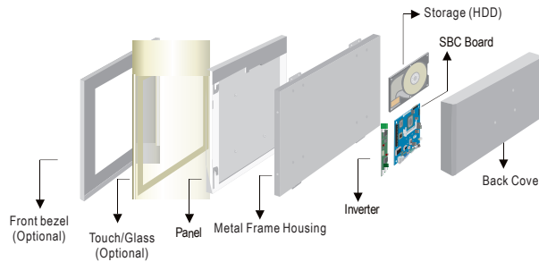
Mechanical design
