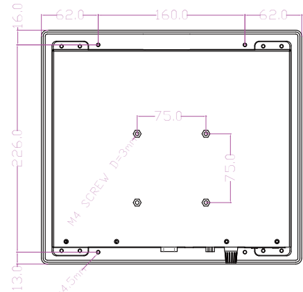
CUT OUT DIMENSION(262x218mm)
