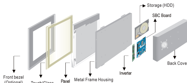
Mechanical design
