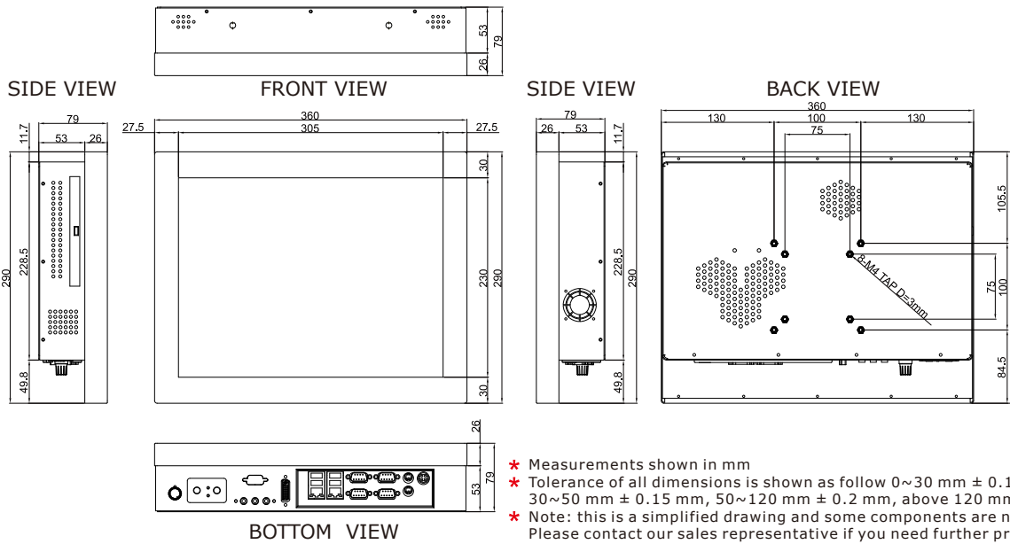
Mechanical design
