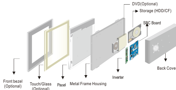
Mechanical design
