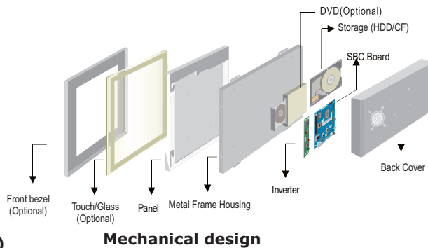
Mechanical design
