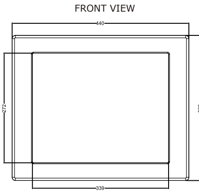
Panel Mount (8 mm front bezel)
