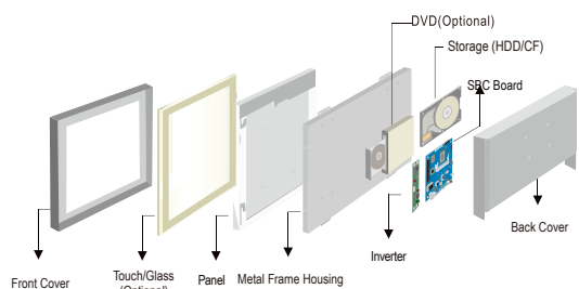
Mechanical design
