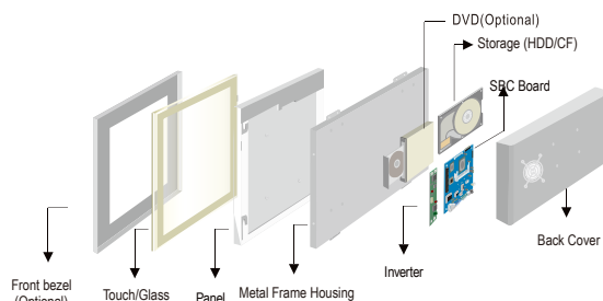
Mechanical design
