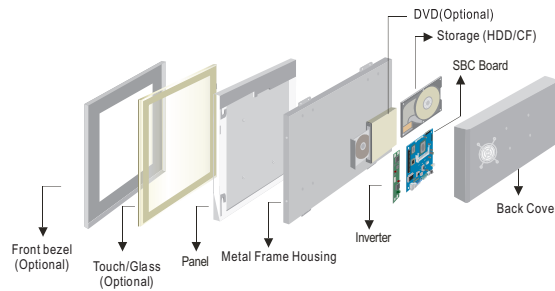
Mechanical design
