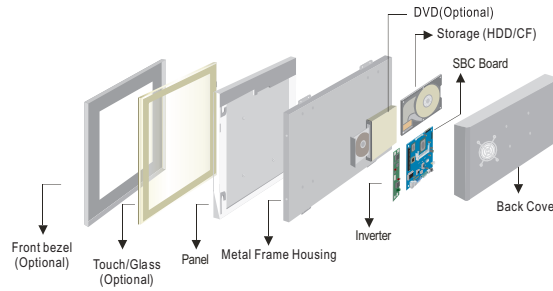
Mechanical design
