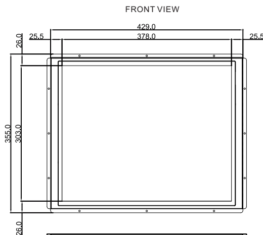
Mechanical design Dimensions
