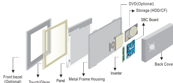
Mechanical design
