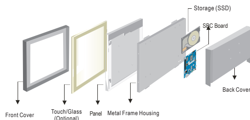
Mechanical design
