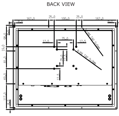
Mechanical design Dimensions
