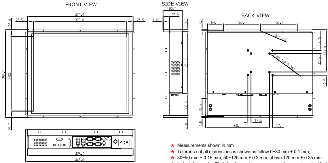
BOTTOM VIEW
