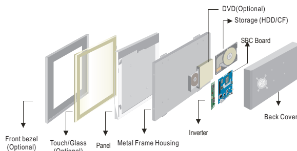
Mechanical design
