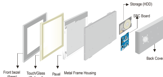
Modularized Construction
