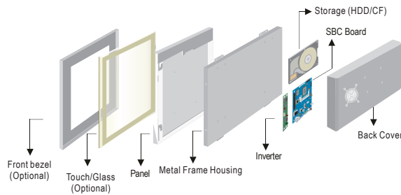
Mechanical design
