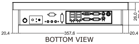
BOTTOM VIEW
