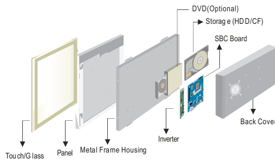
Mechanical design
