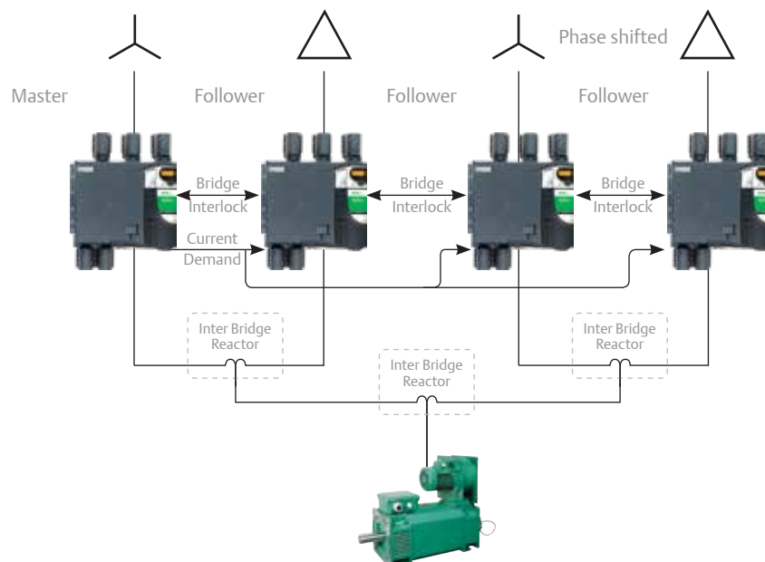
Parallel - 24 pulse
