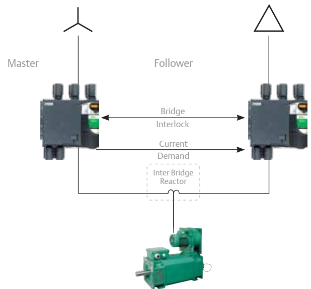
Parallel - 12 pulse
