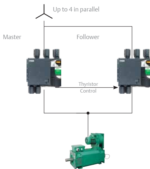
Parallel - 6 pulse
