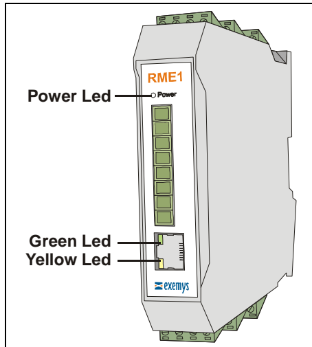
Figure 12 - Leds indicators
