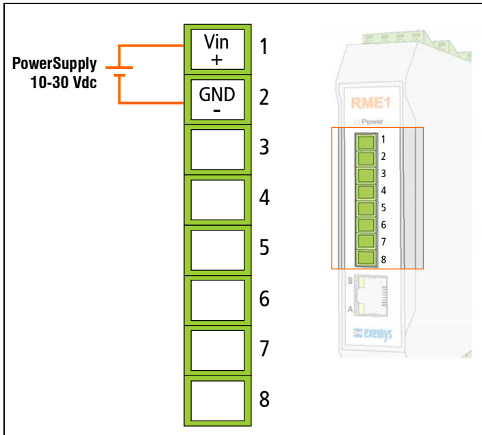
Figure 4 - Power connection diagram
