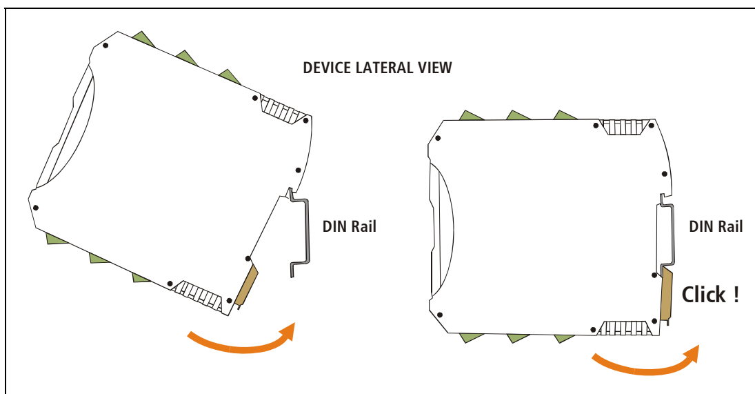
Figure 27 -Device assembly
