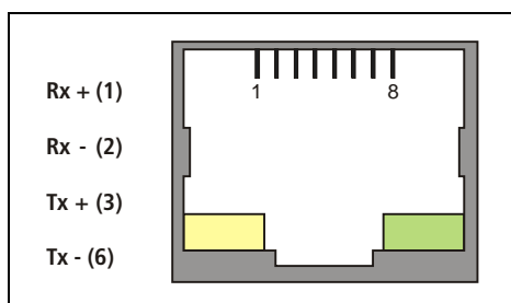
Figure 9 - RJ45 connector
