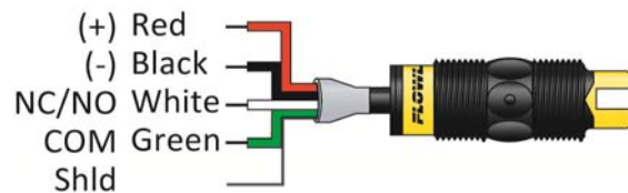
Ultrasonic (LU10-1305 or LU10-1325) Wire Configuration
