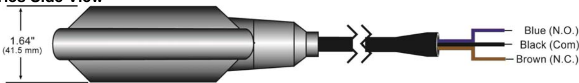
LV42 Series Top View
