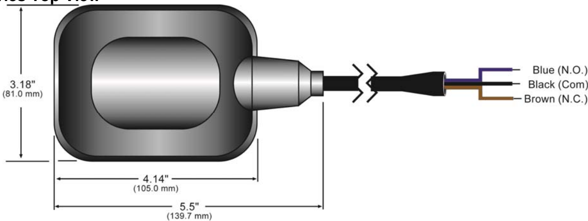
LV41 Series Side View
