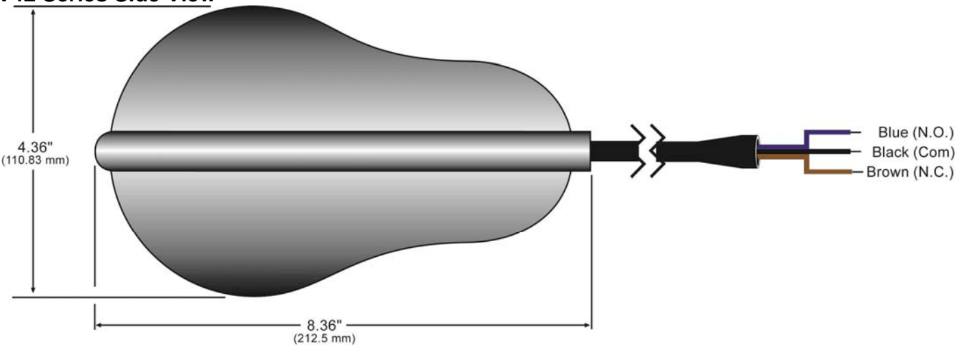
LV42 Series Side View
