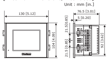
[External Dimensions/Interfaces]
