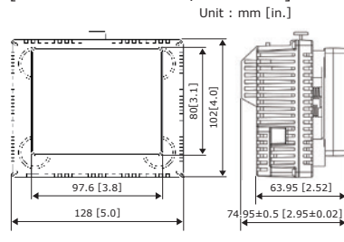
[External Dimensions/Interfaces]
